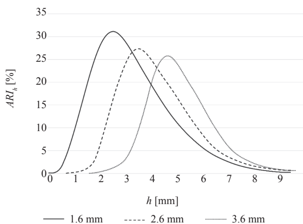
Figure 4 – The distributions that conform to the conditions of the tires of the vehicle fleet at different minimum allowable tire tread depths
