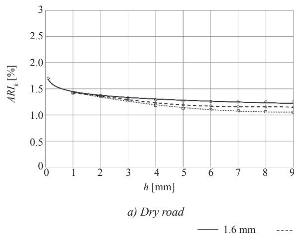
Figure 5 – Prediction of accident rate of used vehicle fleet according to the different requirements to the permissible minimum tire tread depth
