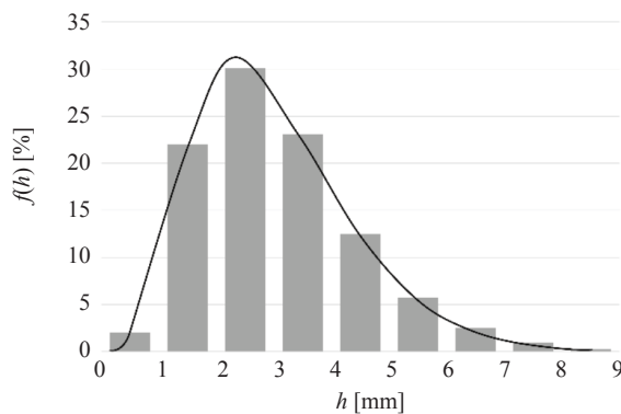
a) Differential statistical model
