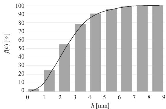
b) Integral statistical model
