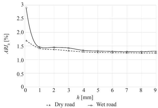
Figure 3 – The statistical model of road accident probability depending on tire tread depth
