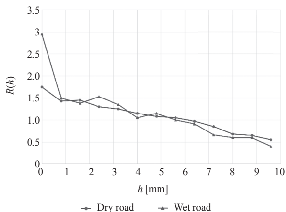
Figure 2 – Dependence of risk index on tire tread depth [43, 44]
