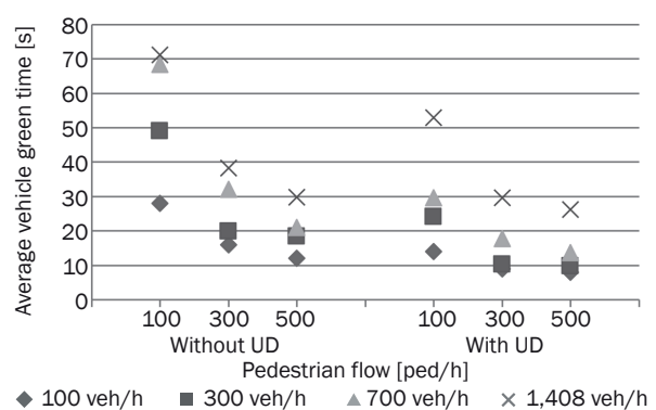
Figure 6 – Change in the average vehicle green time with Upstream Detection (UD)
