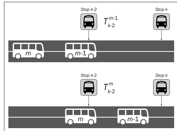
Figure 3 - Illustration of d_3 (T_{k-2}^{m-1}) and d_4 (T_{k-2}^m)
